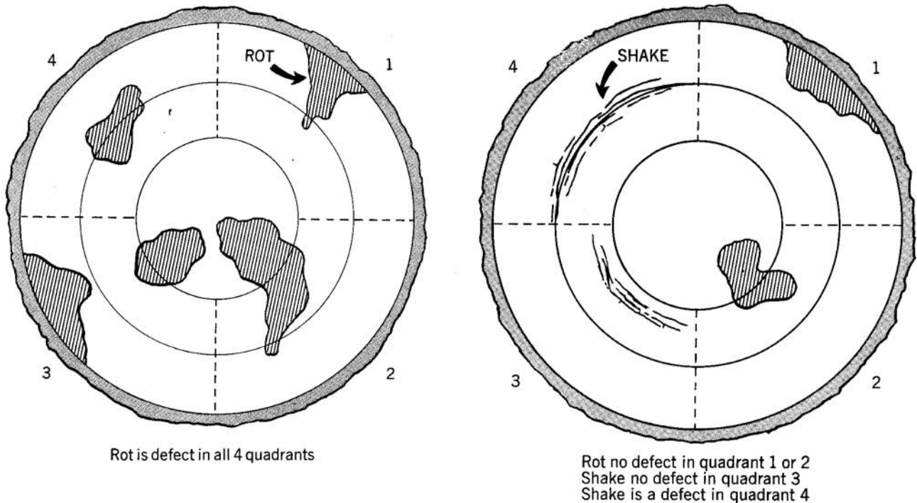
Figure 13.—Evaluation of rot and shake in hardwood factory lumber logs.
