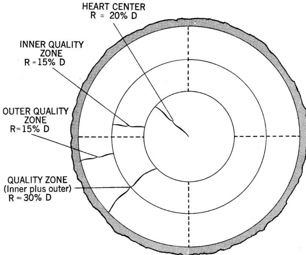
Figure 12.—Location of end features in hardwood factory lumber logs.
